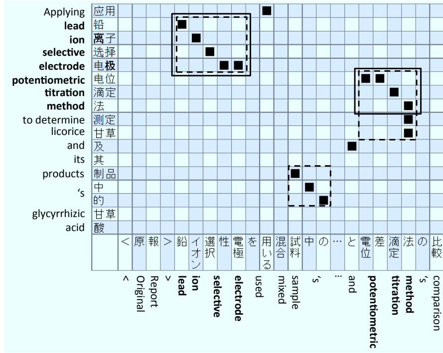
Figure 2: Example of comparable sentences with alignment results computed by IBM models (Parallel fragment candidates are in dashed rectangles, parallel fragments are in rectangles with solid line border).
